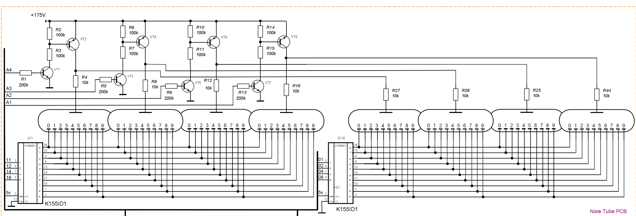
Nixie Tube PCB
